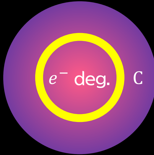
Shell C ignition
