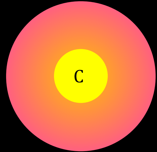
Core C ignition
